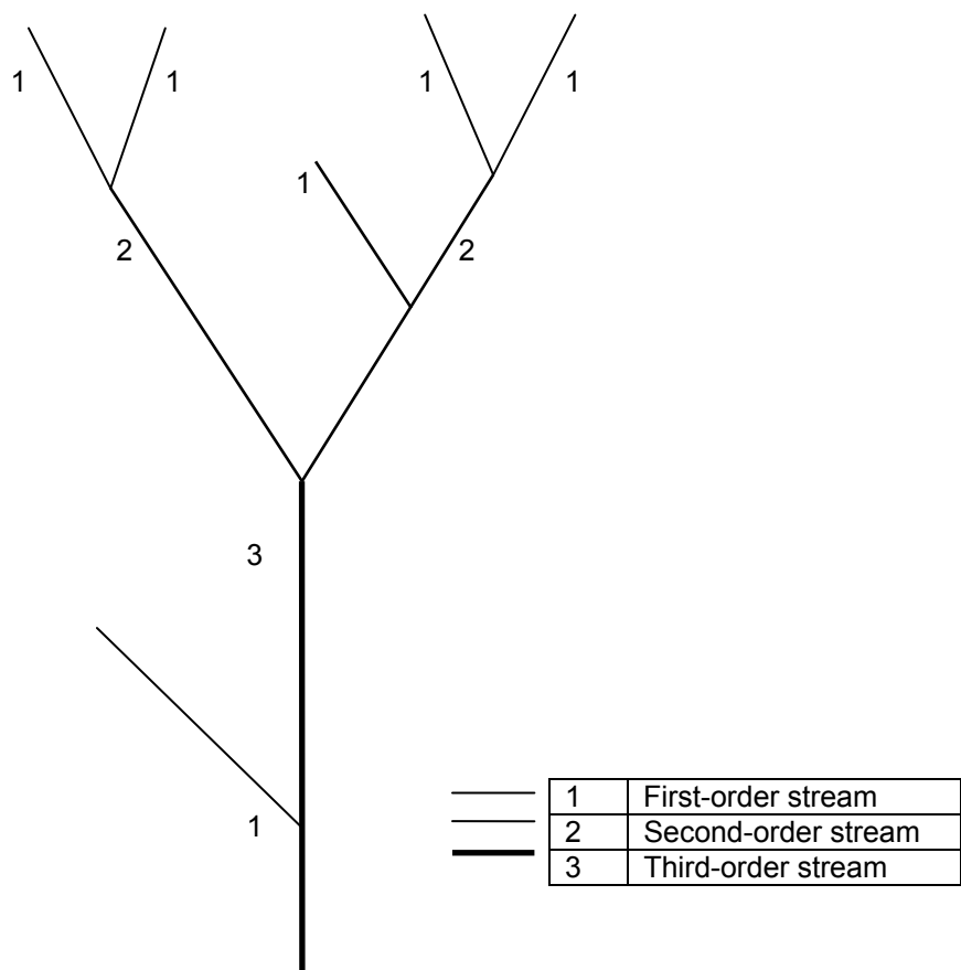
Figure 3: Schematic diagram of stream order (after Strahler 1964)
